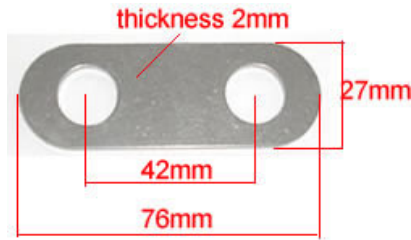
JOINT PLATE PUMP TSUDAKOMA ZW 603668
