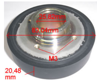
BLACK ROLLER TO PRESS THE PICK NISSAN LW/TSU
