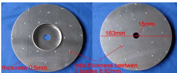
TURBINE TSUDAKOMA ZW 163x15x8,92mm
