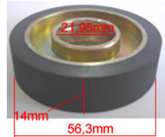
PRESSURE ROLLER D=56,3mm NISSAN LW/TSUDAK.ZW
