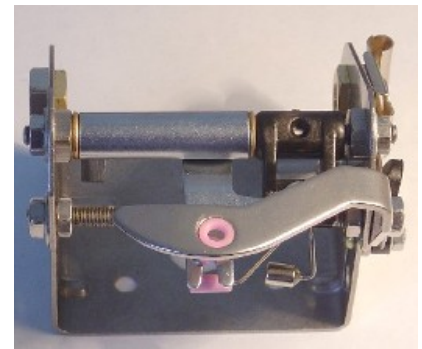
LENO DEVICES TZUDAKOMA ZA205/209/ZAX LX 620302-57
