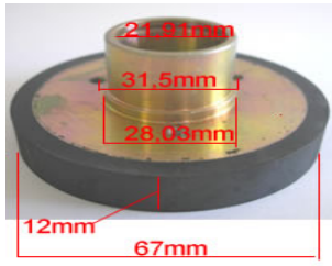
ROLLER FOR FEEDER TSUD.ZW/NISSAN LW/TOYOTA
