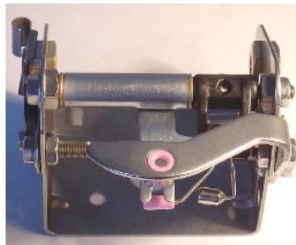
BOBIN HOLDER ASSY TZUDAKOMA ZA205/209/ZAX RH
