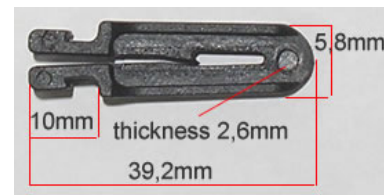
HOOK REGGIL. NISSAN/TSUD. 39,2X10X5,8X2,6 DH-S0300-0
