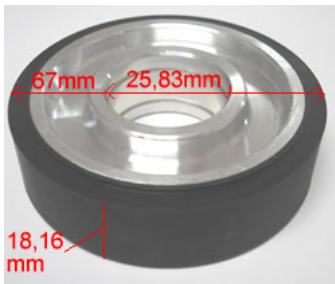
BLACK ROLLER TO PRESS THE PICK NISSAN LW/TSU EM-059A0-0
